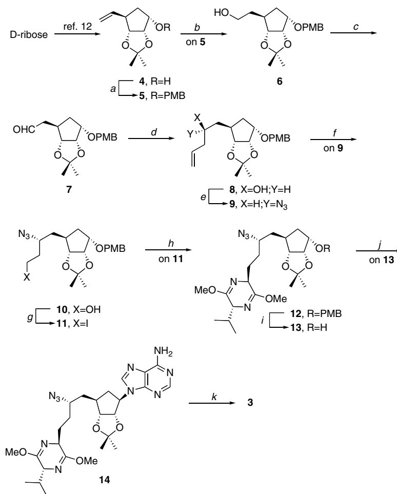
Scheme 1. Reagents and conditions: (a) PMBCl, NaH, DMF, 95%; (b) (i) 9-BBN, THF; (ii) MeOH, H 2 O 2 , NaOH, 98% for two steps; (c) SO 3 ·py, DMSO, DIPEA, CH 2 Cl 2 , 94%; (d) (i) (+)-B-methoxydiisopinocampheylborane, CH 2 =CHCH 2 MgBr, Et 2 O/THF; (ii) MeOH, H 2 O 2 , NaOH, 96% for two steps; (e) (i) MsCl, Et 3 N, DMAP, CH 2 Cl 2 ; (ii) NaN 3 , DMF, 85% for two steps; (f) (i) NaIO 4 , OsO 4 , MeOH/H 2 O; (ii) NaBH 4 , CeCl 3 ·7 H 2 O, MeOH, 77% for two steps; (g) TPP, imidazole, I 2 , toluene/MeCN, 90%; (h) (2 R )-3,6-dihydro-2,5-dimethoxy-3-isopropylpyrazine, BuLi, CuCN, THF, 87%; (i) DDQ, CH 2 Cl 2 /H 2 O, 88%; (j) (i) Tf 2 O, pyridine, CH 2 Cl 2 ; (ii) adenine, NaH, DMF, 45% for two steps; (k) (i) 0.5 N HCl MeOH; (ii) Pd(OH) 2 /C, cyclohexene; (iii) LiOH, MeOH/H 2 O, 55% for three steps.
