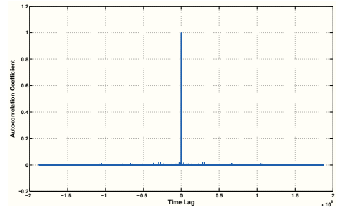
Fig. 4. Correlation between time ordered delay samples.
