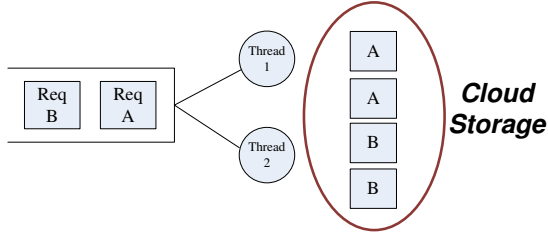
Fig. 5. An example of a two-thread queue
