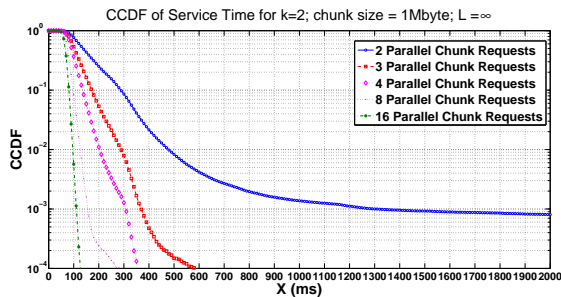
Fig. 11. Complementary cumulative distribution function (CCDF) of service time with unlimited bandwidth for a 2Mbyte file and k=2 .
