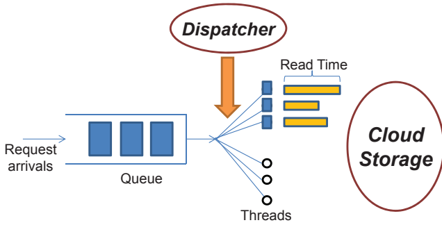
Fig. 2. The architecture for data retrieval through a multiple-thread dispatcher.
