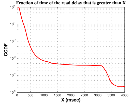
Fig. 3. CCDF of read delay for 1MB chunk.
