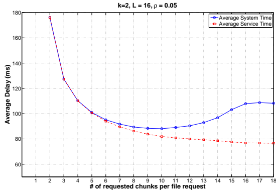
Fig. 10. Greedy scheme is not delay-optimal in general over real clouds.
