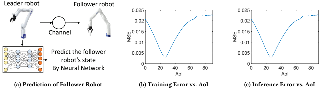
Figure 2: Robot state prediction in a leader-follower robotic system. The leader robot uses a neural network to predict the follower robot's state. The training and inference errors decrease in the AoI \leq 25 and increase when AoI \geq 25 .
