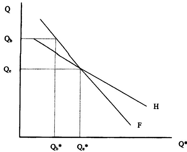
Fig. 1. Nash equilibrium and quota constrained outputs.
