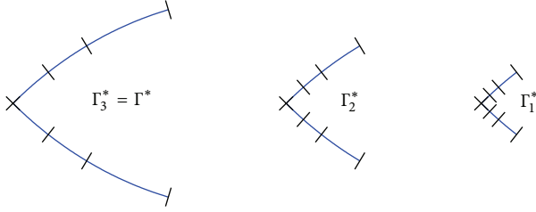
FIGURE 5: The boundary subsets \Gamma_3^* , \Gamma_2^* , and \Gamma_1^* along with their corresponding type b meshes for n_{\text{sub}} = 3 .
