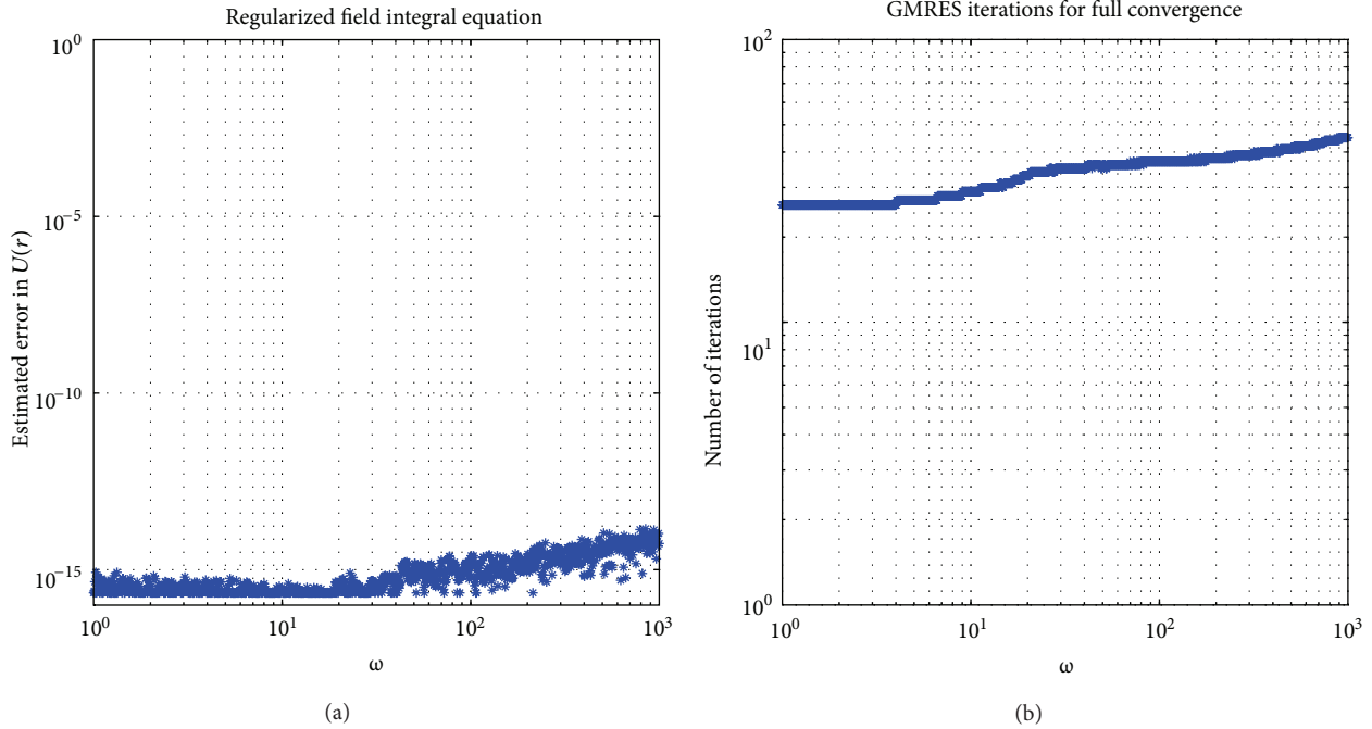
FIGURE 16: The same exterior Neumann problem for Helmholtz equation as in Figure 15, but RCIP is now applied to (68). The program demo13b.m is used.
