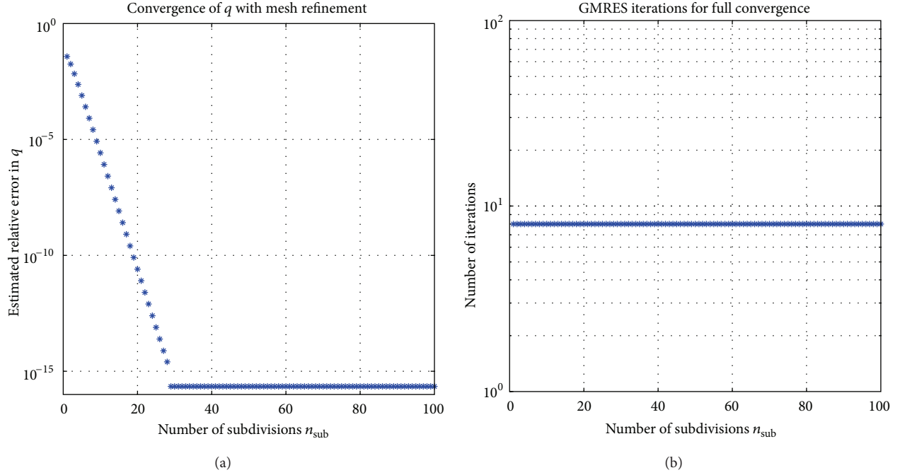
FIGURE 10: Same as Figure 7, but the program demo8b.m is used.
