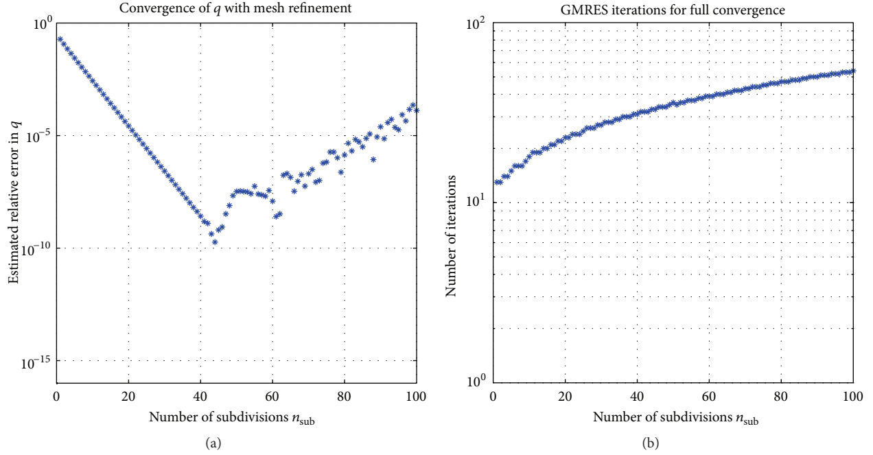
FIGURE 3: Convergence for q of (6) using (8) and the program demo1b.m (a loop of demo1.m ) with \lambda = 0.999 , \theta = \pi/2 , n_{\text{pan}} = 10 , and \text{evc} = 1 . The reference value is q = 1.1300163213105365 . There are n_p = 160 + 32n_{\text{sub}} unknowns in the main linear system. (a) Convergence with n_{\text{sub}} . (b) The number of iterations needed to meet an estimated relative residual of \epsilon_{\text{mach}} .
