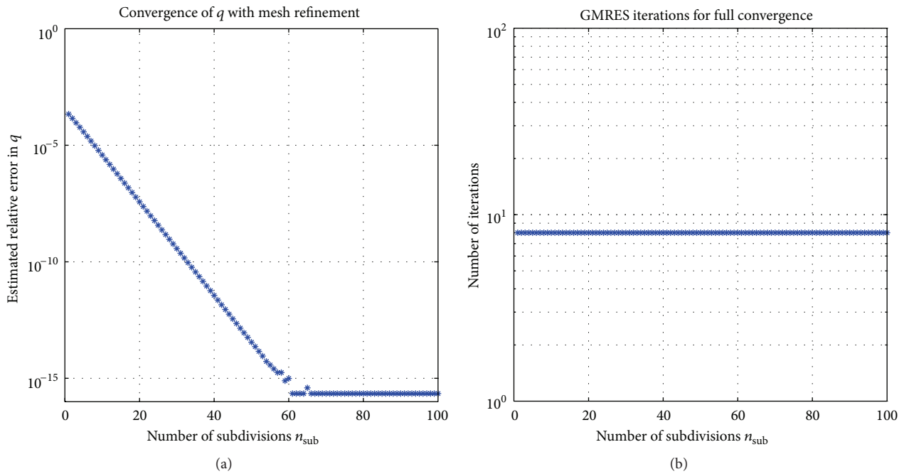
FIGURE 7: Same as Figure 6, but the program demo3b.m is used.
