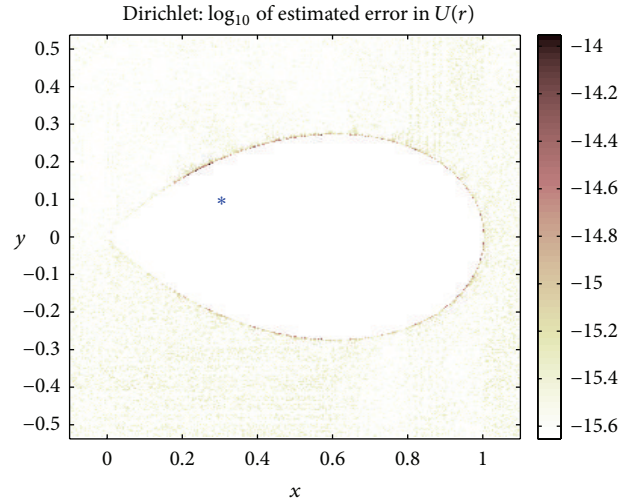
FIGURE 17: The error in the solution U(r) to the exterior Dirichlet Helmholtz problem of Section 16 evaluated at 62392 points on a cartesian grid using demo11b.m with \omega = 10 . The source at r' = (0.3, 0.1) is shown as a blue star.
