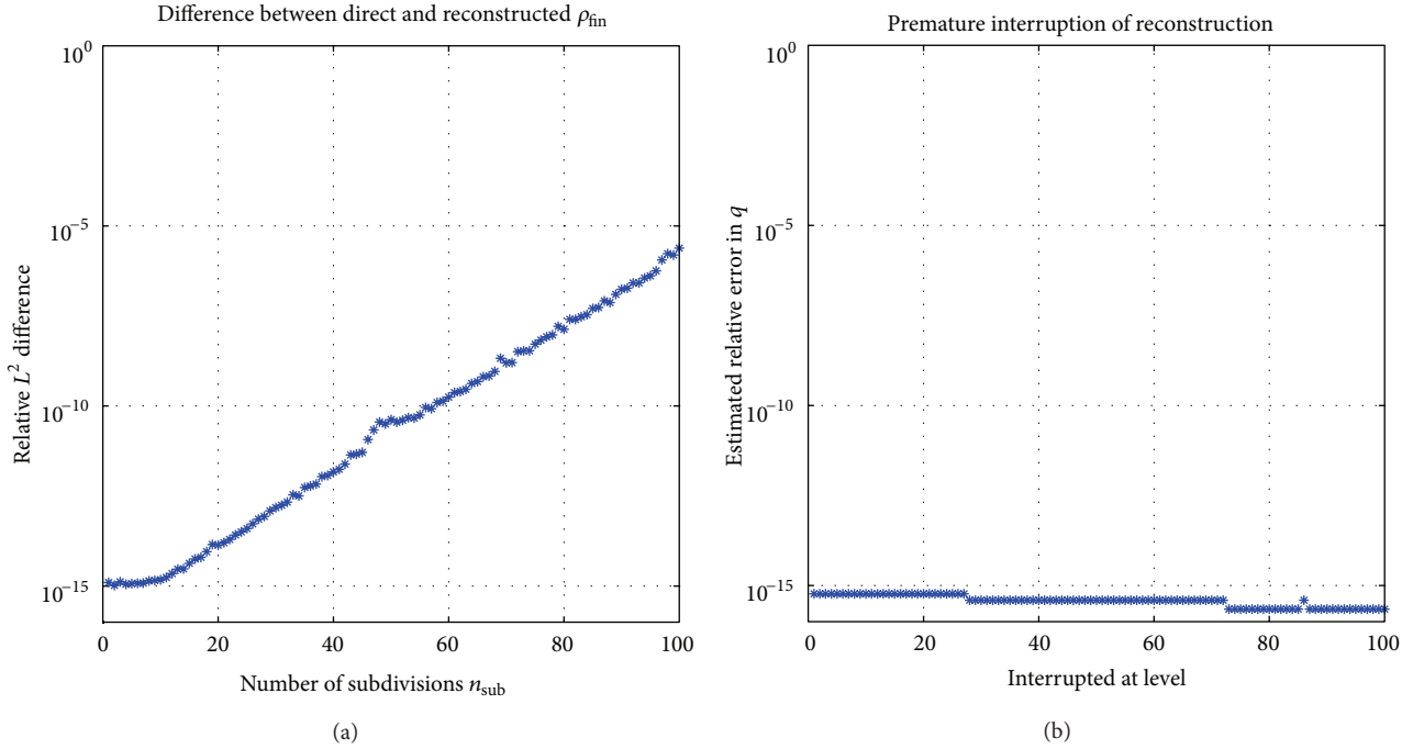
FIGURE 8: Output from demo4.m and demo5.m . (a) A comparison of \rho_{\text{fin}} from the unstable equation (8) and \rho_{\text{fin}} reconstructed from \tilde{\rho}_{\text{coa}} of (17) via (33). (b) Relative accuracy in q of (6) from part-way reconstructed solutions \tilde{\rho}_{\text{part}} .
