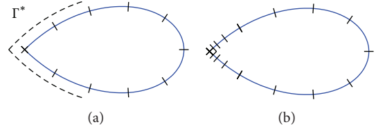
FIGURE 2: (a) A coarse mesh with ten panels on the contour \Gamma of (1) with opening angle \theta = \pi/2 . A subset of \Gamma , called \Gamma^* , covers four coarse panels as indicated by the dashed curve. (b) A fine mesh created from the coarse mesh by subdividing the panels closest to the corner n_{\text{sub}} = 3 times.
