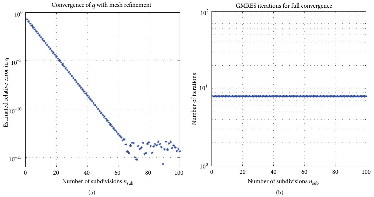
FIGURE 6: Same as Figure 3, but using (17) and the program demo2b.m (a loop of demo2.m ). There are only n_p = 160 unknowns in the main linear system.
