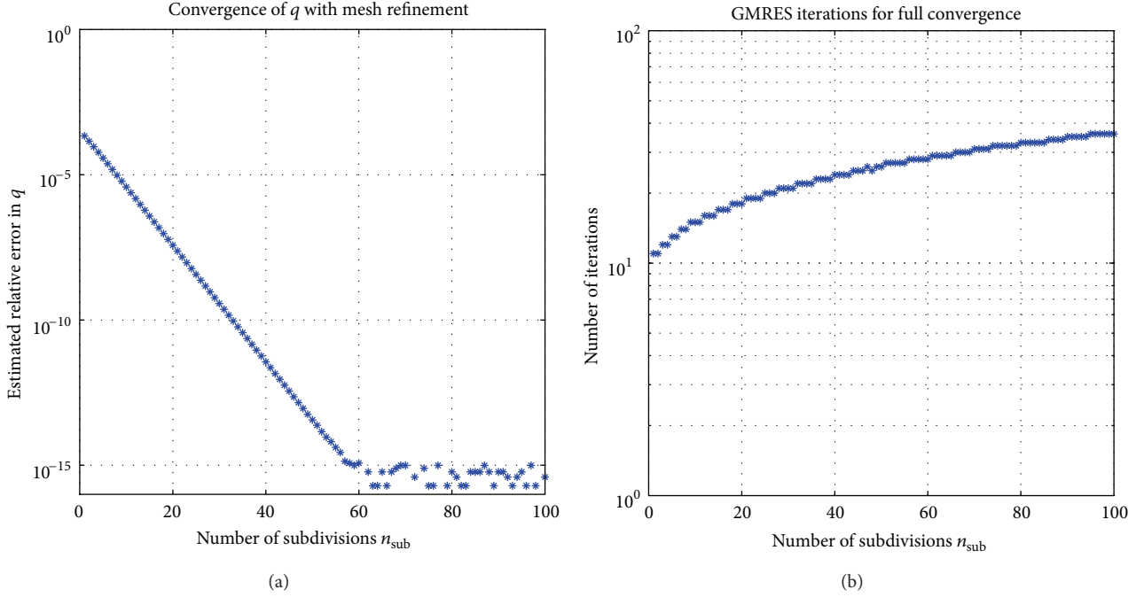
FIGURE 20: Same as Figure 7, but the program demo1d.m is used.
