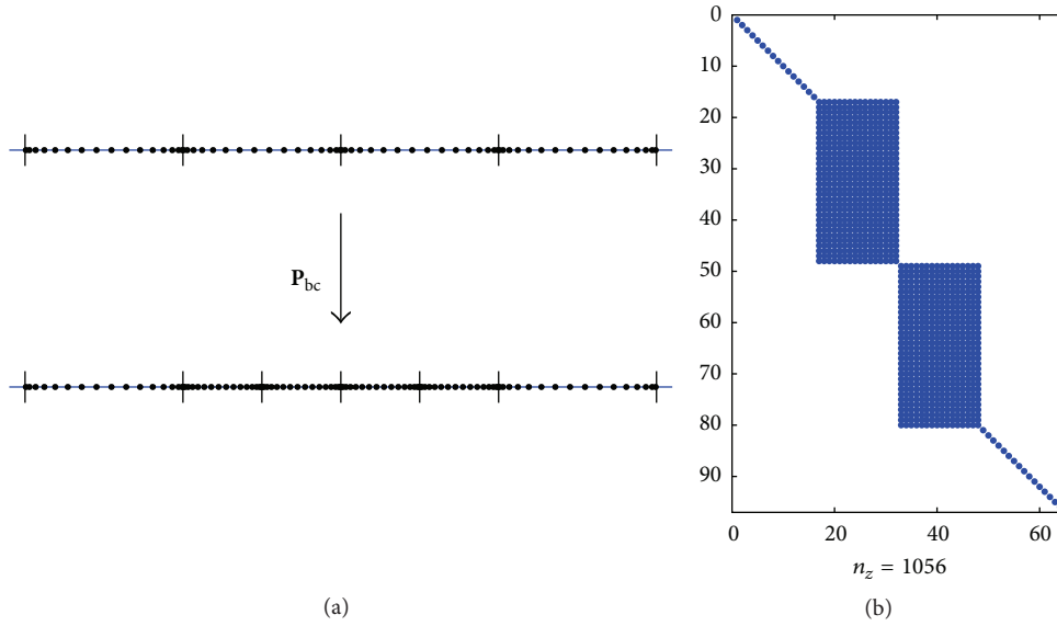
FIGURE 4: (a) The prolongation operator \mathbf{P}_{bc} performs panelwise interpolation from a grid on a four-panel mesh to a grid on a six-panel mesh. (b) The sparsity pattern of \mathbf{P}_{bc} .
