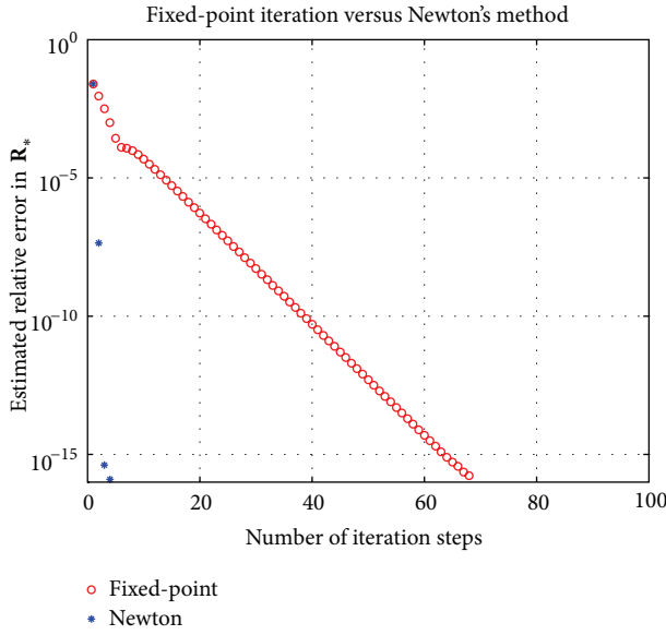
FIGURE 11: Output from the program demo9.m. The fixed-point iteration (36) and (37) is compared to Newton's method for (38).
