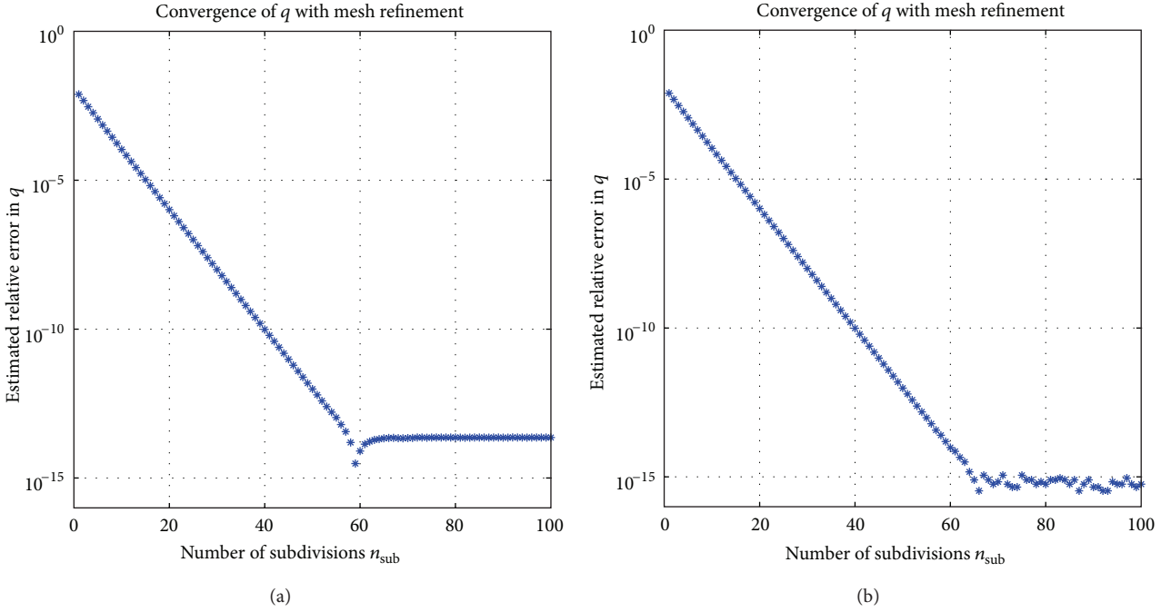
FIGURE 13: Convergence for q of (6) with \rho = \rho_1 from (42). The curve \Gamma is as in (1), and \theta = \pi/2 , n_{\text{pan}} = 11 , and \text{evect} = 1 . The reference value is taken as q = 1.95243329423584 . (a) Results from the inner product preserving scheme of Appendix D produced with demo10.m. (b) Results with RCIP according to (47) and (48) produced with demo10b.m.
