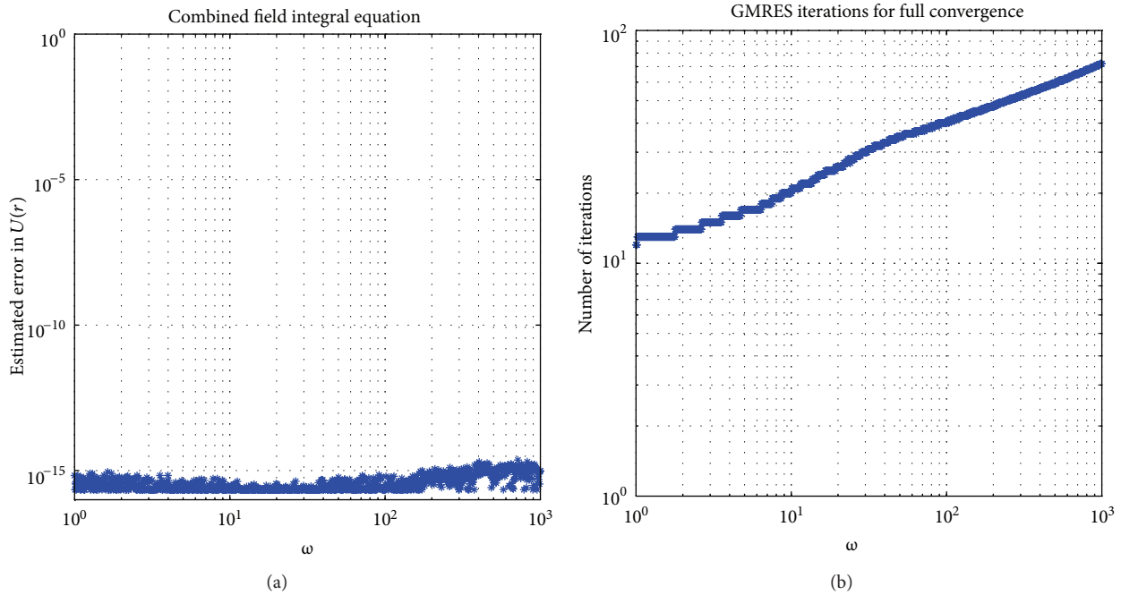
FIGURE 14: The exterior Dirichlet problem for Helmholtz equation with RCIP applied to (55). The program demo11.m is used with \Gamma as in (1), and \theta = \pi/2 . The boundary condition g(r) of (51) is generated by a point source at (0.3, 0.1) . (a) The absolute error in U(r) at r = (-0.1, 0.2) . (b) The number of GMRES iterations needed to meet an estimated relative residual of \epsilon_{\text{mach}} .
