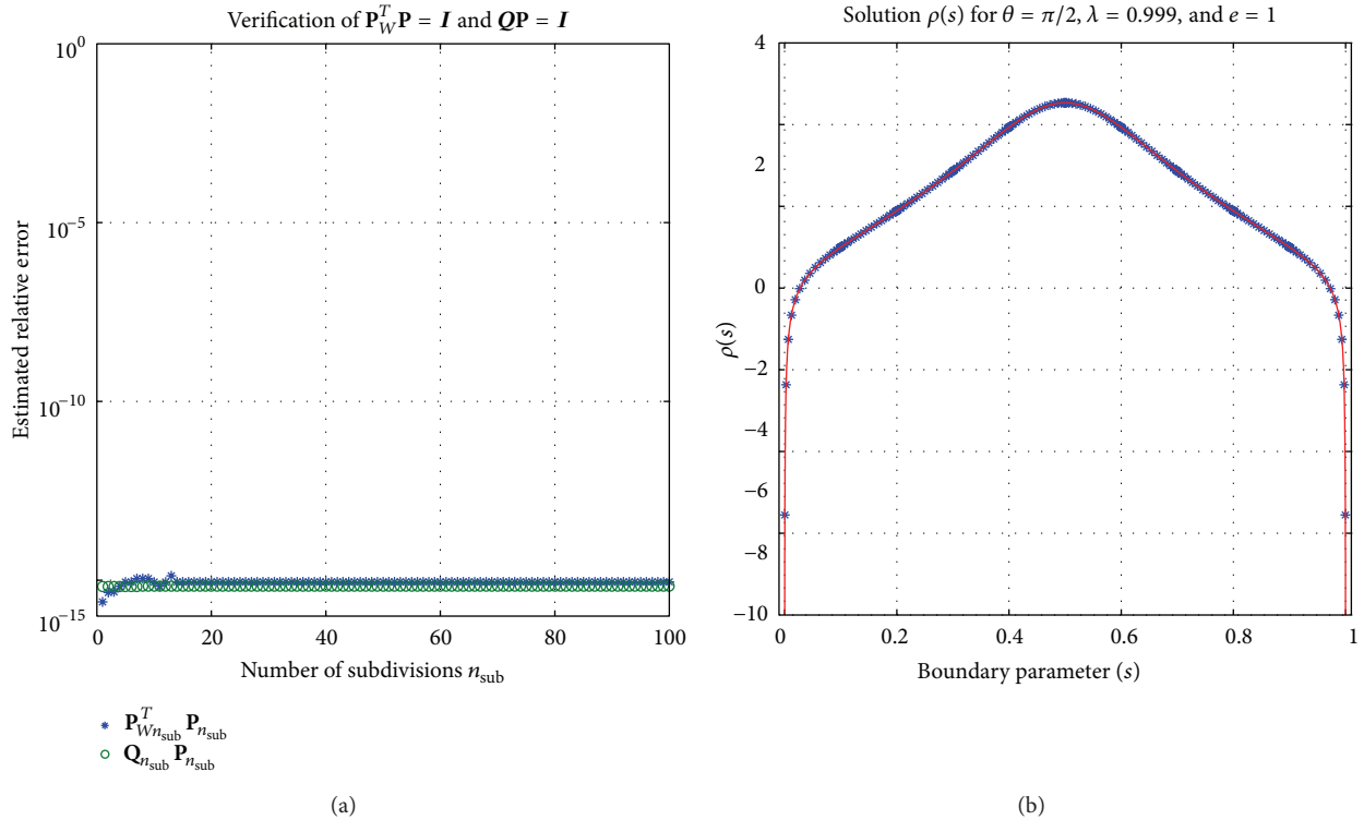
FIGURE 9: (a) The identities (14) and (31) hold to high accuracy in our implementation, irrespective of the degree of mesh refinement. (b) The solution \rho to (25) on (1) with parameters as specified in Section 4. The solution with RCIP (17) and (28), shown as blue stars, agrees with the solution from (8), shown as a red solid line. The solution diverges in the corner.
