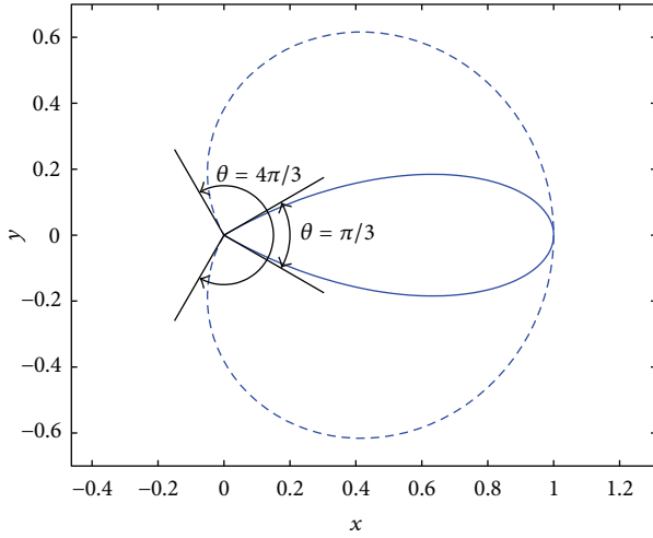
FIGURE 1: The contour \Gamma of (1) with a corner at the origin. The solid curve corresponds to opening angle \theta = \pi/3 . The dashed curve has \theta = 4\pi/3 .
