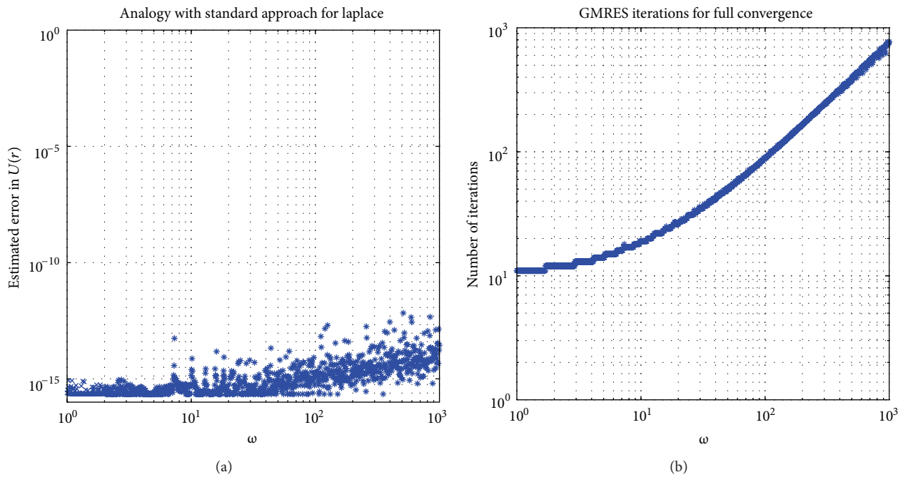
FIGURE 15: The exterior Neumann problem for Helmholtz equation with RCIP applied to (63). The program demo12.m is used with \Gamma as in (1), and \theta = \pi/2 . The boundary condition g(r) of (59) is generated by a point source at (0.3, 0.1) . (a) The absolute error in U(r) at r = (-0.1, 0.2) . (b) The number of GMRES iterations needed to meet an estimated relative residual of \epsilon_{\text{mach}} .
