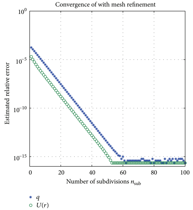
FIGURE 12: Similar as Figure 7(a) but with the program demo3c.m . The potential U(r) at r = (0.4, 0.1) is evaluated via (41), and npan = 14 is used.
