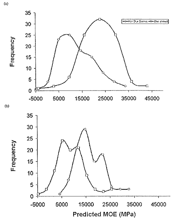
Figure 3. The prediction of MOE for stained ( n=101 ) and unstained ( n=101 ) wood using (a) PCR and (b) PCR from 1 st derivative spectra. Sample set N1S and I1S (Table 1).
