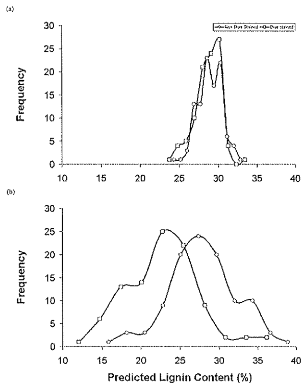
Figure 5. The prediction of lignin for stained ( n=101 ) and unstained ( n=101 ) wood using (a) MLR and (b) PCR. Sample set N1S and I1S (Table 1).
