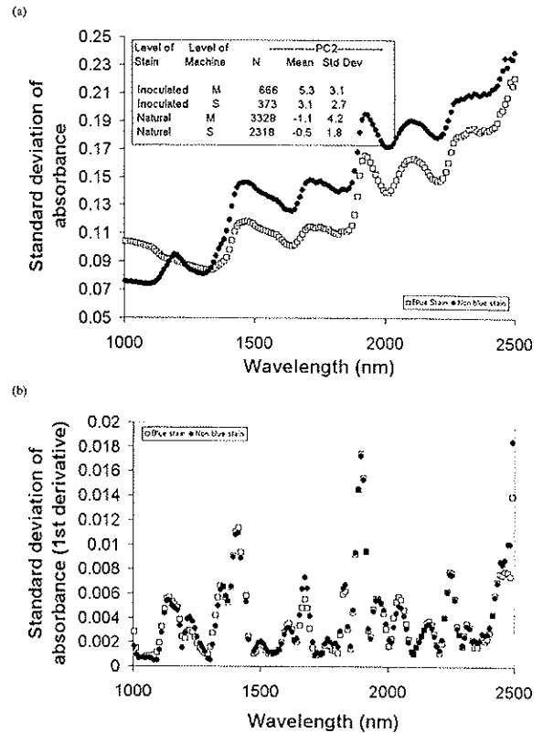
Figure 7. (a) The response in standard deviation of absorbance and PC2 for all levels of stain, instrument, and wavelength. (b) The response in standard deviation of the 1 st derivative of absorbance for natural and inoculated wood for all wavelengths.
