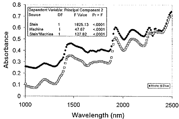
Figure 6. A plot of wavelength versus absorbance for the master and slave along with significance testing of stain, instrument, and stain by instrument along the 2 nd PC.
