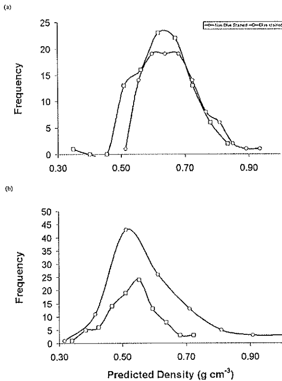
Figure 2. The prediction of density for stained ( n=101 ) and unstained ( n=101 ) wood using (a) PCR and (b) MLR. Sample set N1S and I1S (Table 1).
