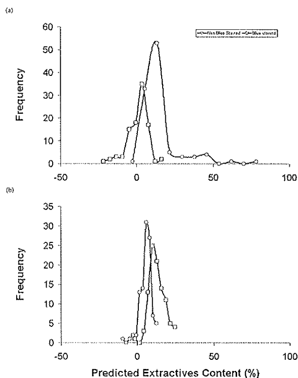
Figure 4. The prediction of extractives for stained ( n=101 ) and unstained ( n=101 ) wood using (a) MLR and (b) PCR from 1 st derivative spectra. Sample set N1S and I1S (Table 1).
