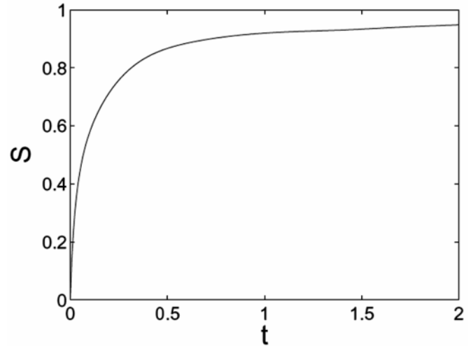
Fig. 3: Linear entropy S (mixedness) as function of time t . Time is in unit of 1/\omega_R .
