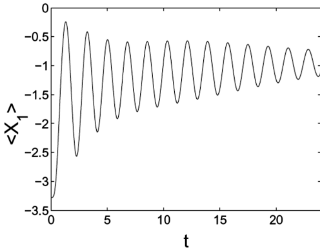
Fig. 1: \langle X_1 \rangle as function of time t . Time is in unit of 1/\omega_R .
