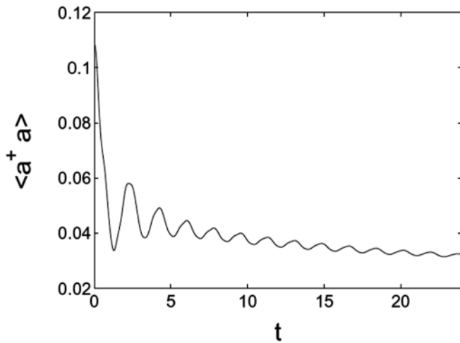
Fig. 2: \langle a^\dagger a \rangle as function of time t . Time is in unit of 1/\omega_R .
