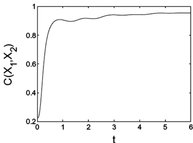
Fig. 4: Covariance C(X_1, X_2) as Function of time t . Time is in unit of 1/\omega_R
