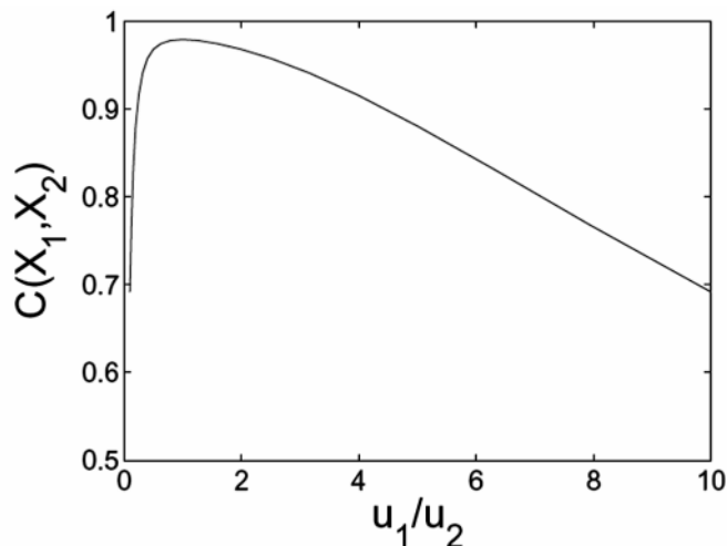
Fig. 5: Covariance C(X_1, X_2) as Function of u_1/u_2 for Fixed u = 169.74\omega_R at t = 24/\omega_R .
