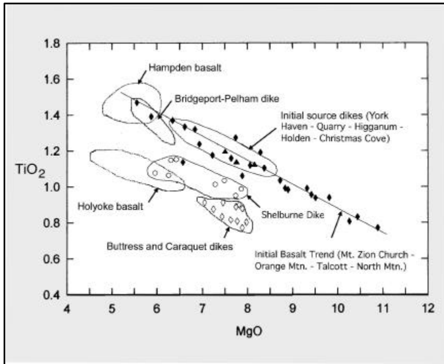
Figure 4. Weight percent TiO 2 -MgO variations in Early Jurassic basalts and dikes in northeastern North America. Compositions of the Ministers Island, Buckman's Creek, New River, and Lepreau River dikes (Table 1) fall within the initial source dikes field (solid triangle symbols) on the North Mountain Basalt trend (defined by solid diamond symbols). Other dikes and basalts are mainly from southern New England. Sources: Philpotts and Martello (1986), McHone (1996), and references cited in Table 1.
