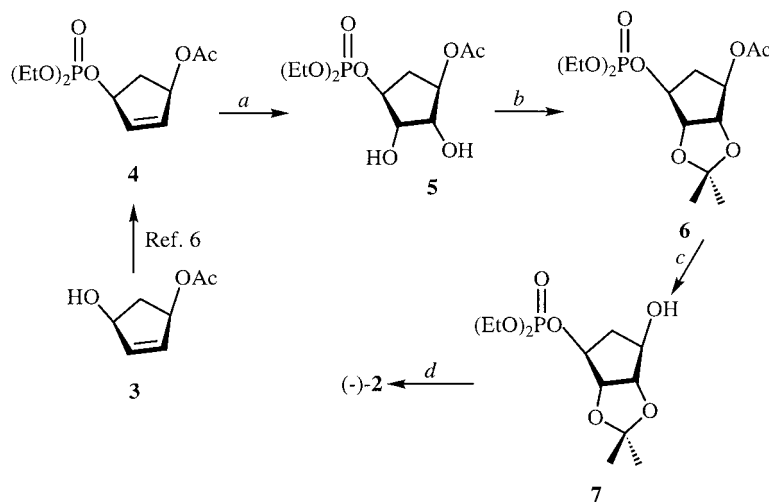
Scheme 2. Reaction conditions: a , N -methylmorpholine N -oxide/catalytic OsO 4 in acetone/H 2 O; b , 2,2-dimethoxypropane/acetone/catalytic p -TsOH; c , NH 3 in MeOH; d , pyridinium chlorochromate and Celite in CH 2 Cl 2 .
