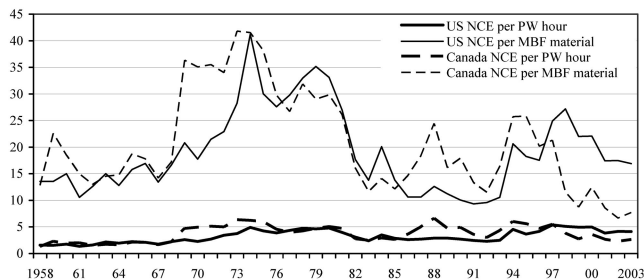
Figure 8. New capital expenditure (NCE) per PW hour and per MBF of material handled (in 2001 US dollars).
