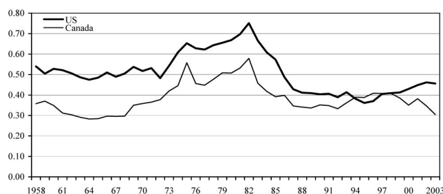
Figure 9. Capital stock per one US dollar of real output (in 2001 US dollars).
