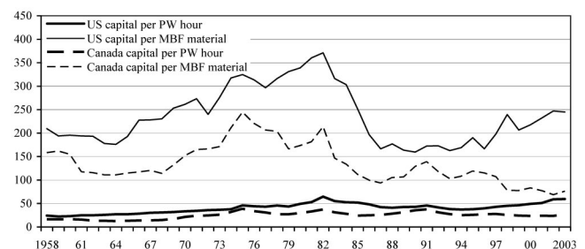
Figure 7. Total capital stock per production worker (PW) hour and per thousand board feet (MBF) of material handled (in 2001 US dollars).
